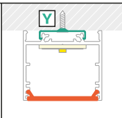
cone Y flexible mounting plate
