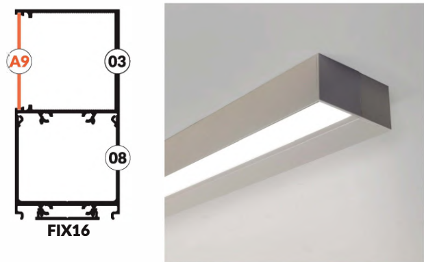
variant 32 - wall side FIX16-08-03-A9
