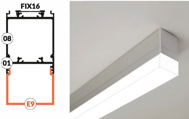
variant 15 - ceiling FIX16-08-01-E9
