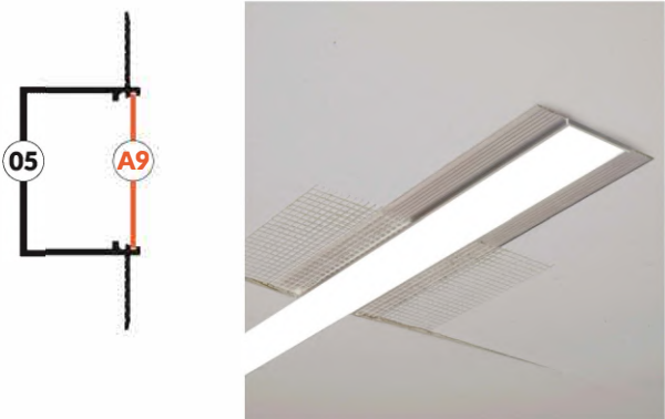
variant 05 - recessed 05-A9 spackle mounting
