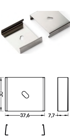
U9 mounting plate material: stainless steel
