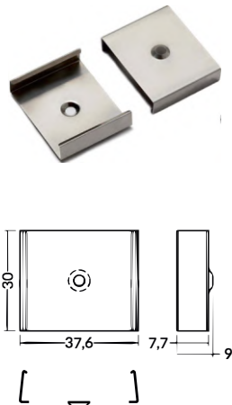
cone U9 mounting plate material: stainless steel
