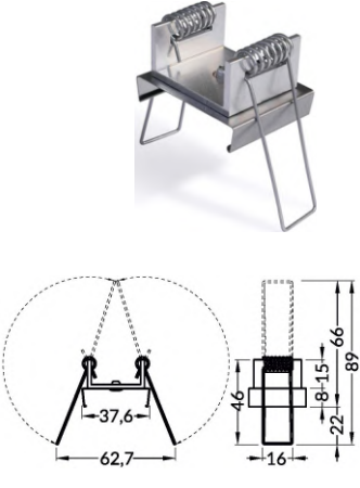
spring U9 mounting plate material: stainless steel, aluminium
