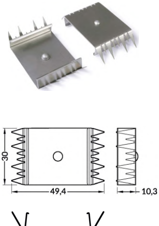
rack U9 mounting plate material: stainless steel
