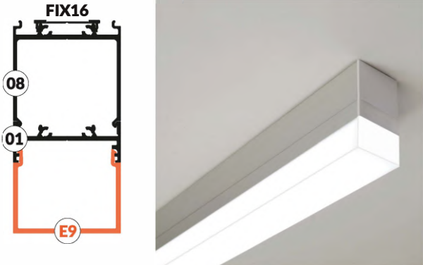
variant 15 - ceiling FIX16-08-01-E9
