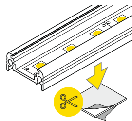
two-sided adhesive tape 25x25
