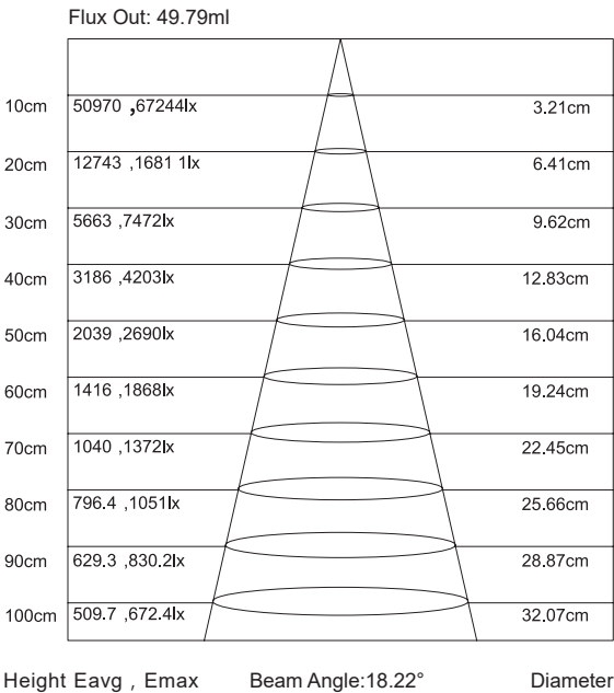
Average Illumination
