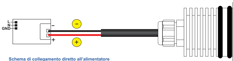
Direct connection diagram to power supply
